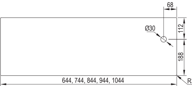
Centre protection panel with holes for economy lock
