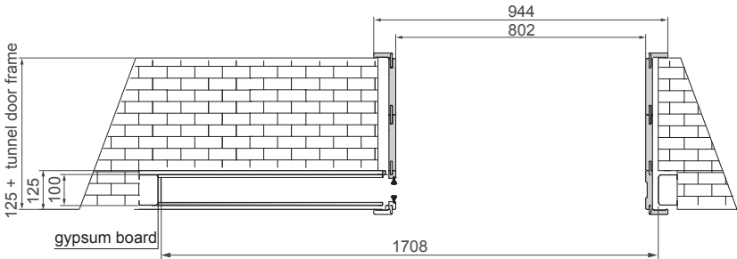
DOOR FRAME RANGE (200-220) TO (400-420) – ASYMMETRIC
