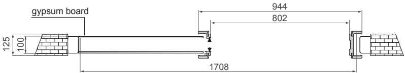
DOOR FRAME RANGE 125 – FIXED
