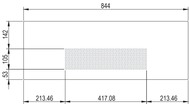
Steel ventilation grill
