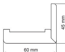
Square to adjustable frame - width 60 mm
