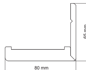
Square to adjustable frame - width 80 mm
