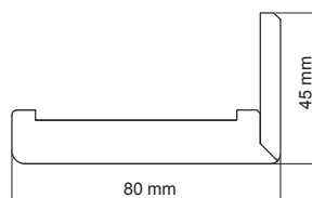
Square to adjustable frame - width 80 mm
