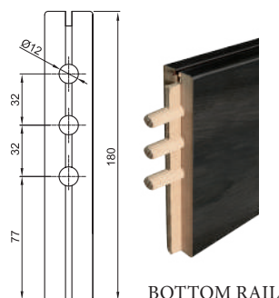
BOTTOM RAIL
