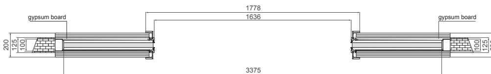
Door frame connection: 45°
