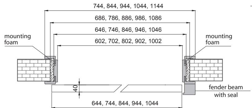
FENDER BEAM
