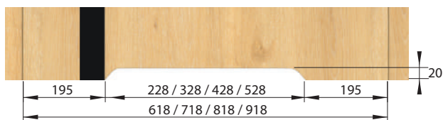
VENTILATION CUT OF DOOR WING MODERNO
