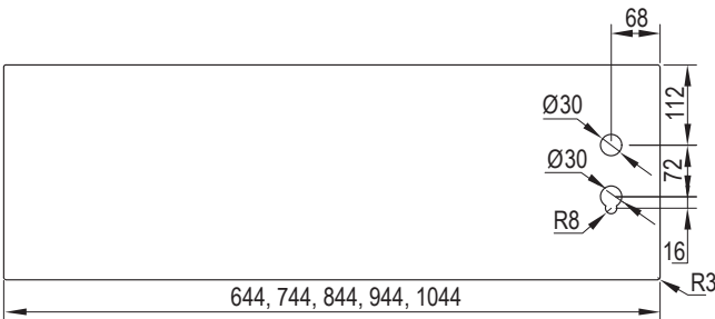
Centre protection panel with holes for bathroom/key lock/cylinder
