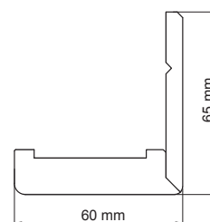
Square to adjustable frame - width 60 mm
