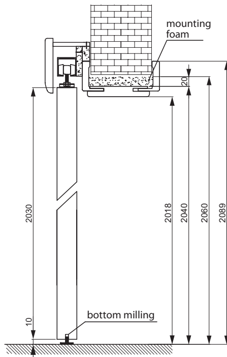
TUNNEL MOUNTING
