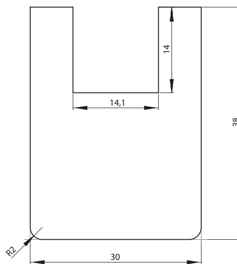
DECORATIVE PROFILES (length 2800)
