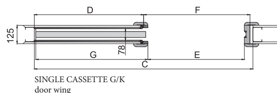
Cassette G/K – single aluminium sliding system
