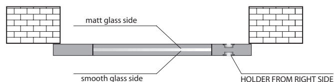
NON-REBATED LEFT (SLIDING TO THE LEFT) DOOR WING
