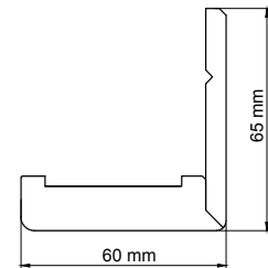
Square to adjustable frame - width 60 mm
