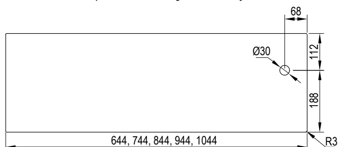
Protective central panel with drilling for economy lock
